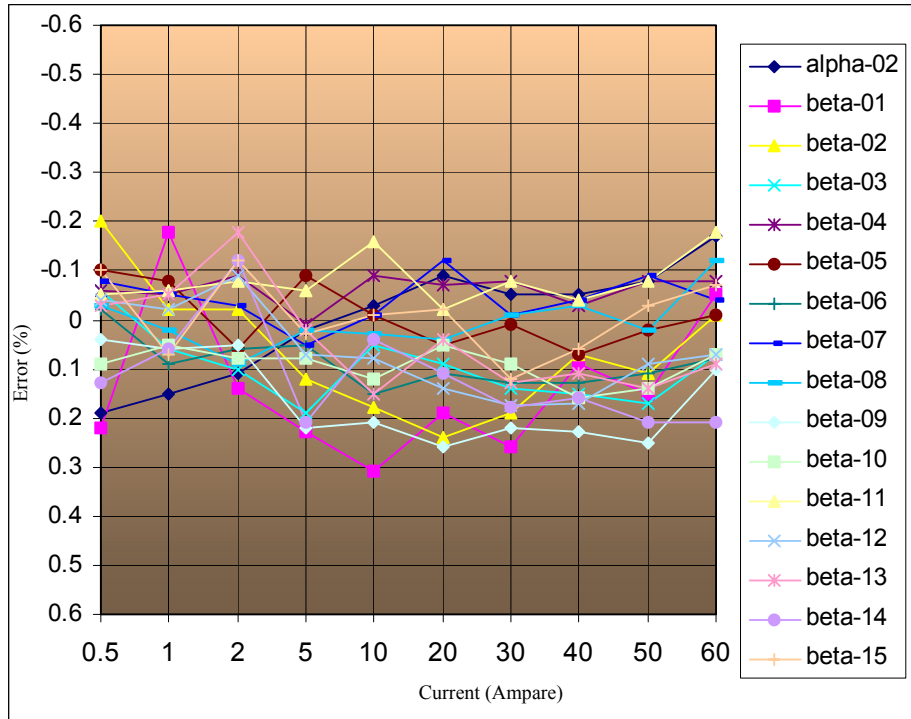
Figure 3 0.8Lead Power Factor (323.3°) Error in %
