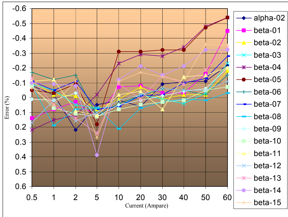
Figure 2 0.5Lag Power Factor (60°) Error in %
