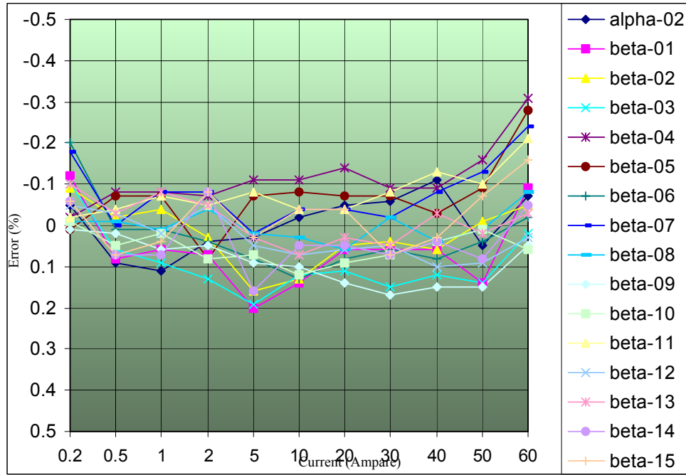
Figure 1 Unity Power Factor (0°) Error in %
